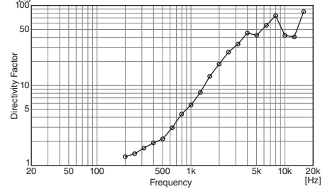
Directivity Factor vs. Frequency
