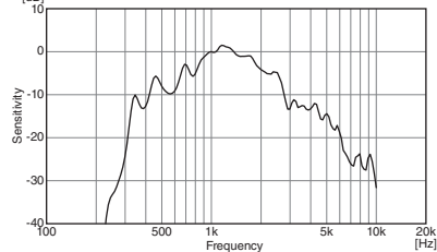
Frequency Response
