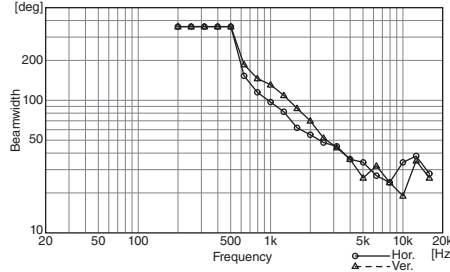
Beamwidth vs. Frequency (-6dB down point)
