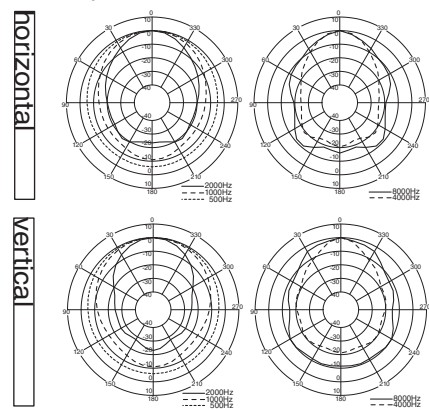
Polar Response
