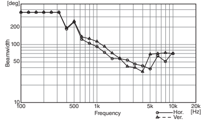
Beamwidth vs. Frequency (-6dB down point)
