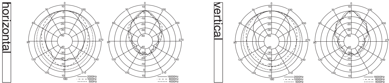
Polar Response
